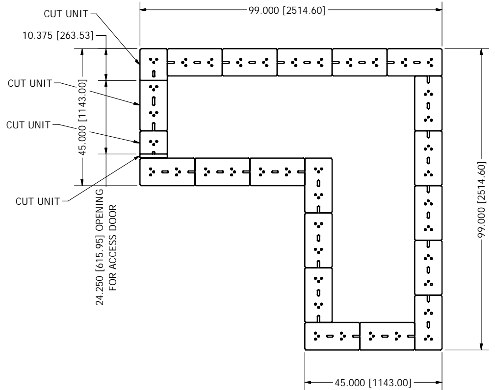
PLAN VIEW
