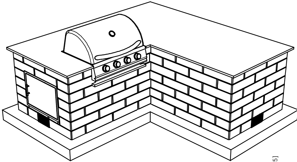
ISOMETRIC VIEW
